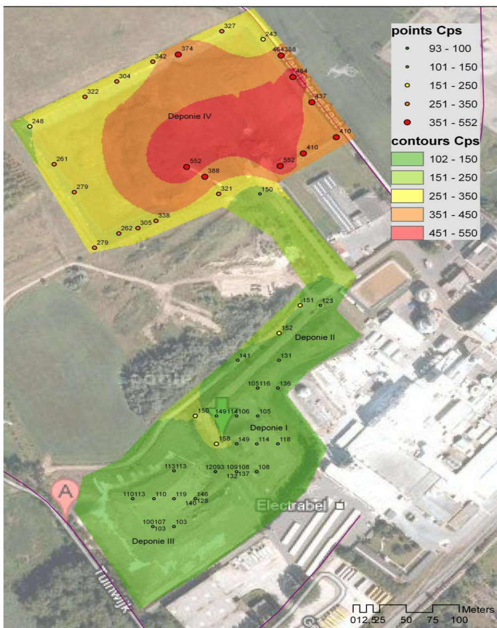
Fig. 4: gamma measurements (in counts per second) at the surface of the landfills of KRONOS EUROPE in Ghent.
