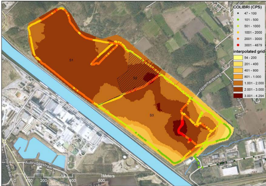
Fig. 1: Gamma radiation count rate (in counts per second) at the surface of mono-landfill "Veldhoven" of TESSENDERLO CHEMIE.
