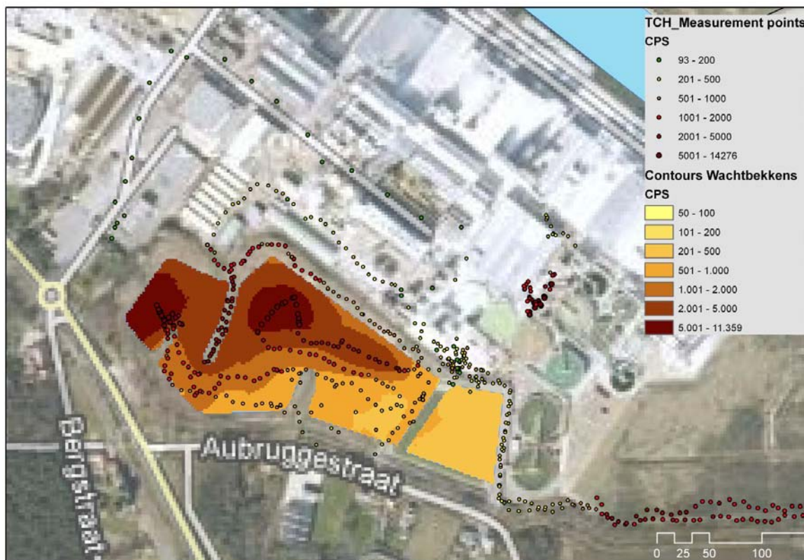
Fig. 3: External gamma radiation (in counts per second) at the surface of a former waste water retention basin at the TESSENDERLO CHEMIE site at Ham.
