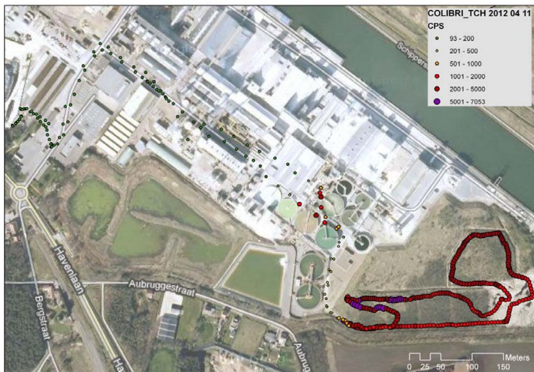
Fig. 2: Gamma count rate (in counts per second) at the surface of the former sludge basin within the premises of the TESSENDERLO CHEMIE site at Ham.
