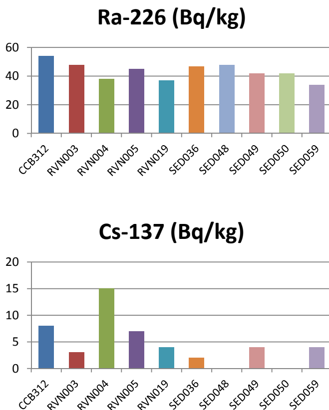
Fig. : activity concentration of radium-226 and cesium-137 in sediments of Walloon watercourses.
