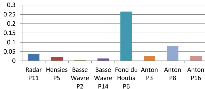
Value of Ra-226 activity concentration measured in the piezometers of the investigated landfills.
