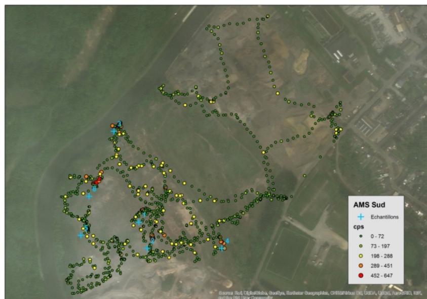
External radiation level at the surface of the site « AMS Sud ». In yellow, orange and red, the points for which the external radiation level exceeds respectively two, three and four times the background level. The crosses shows the sampling points.
