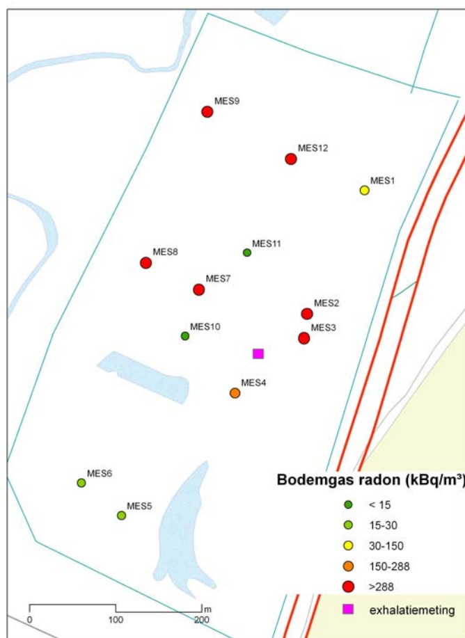
Fig. 4: radon concentration measurements in the soil of the phosphor gypsum disposal site ‘Hoeykens’
