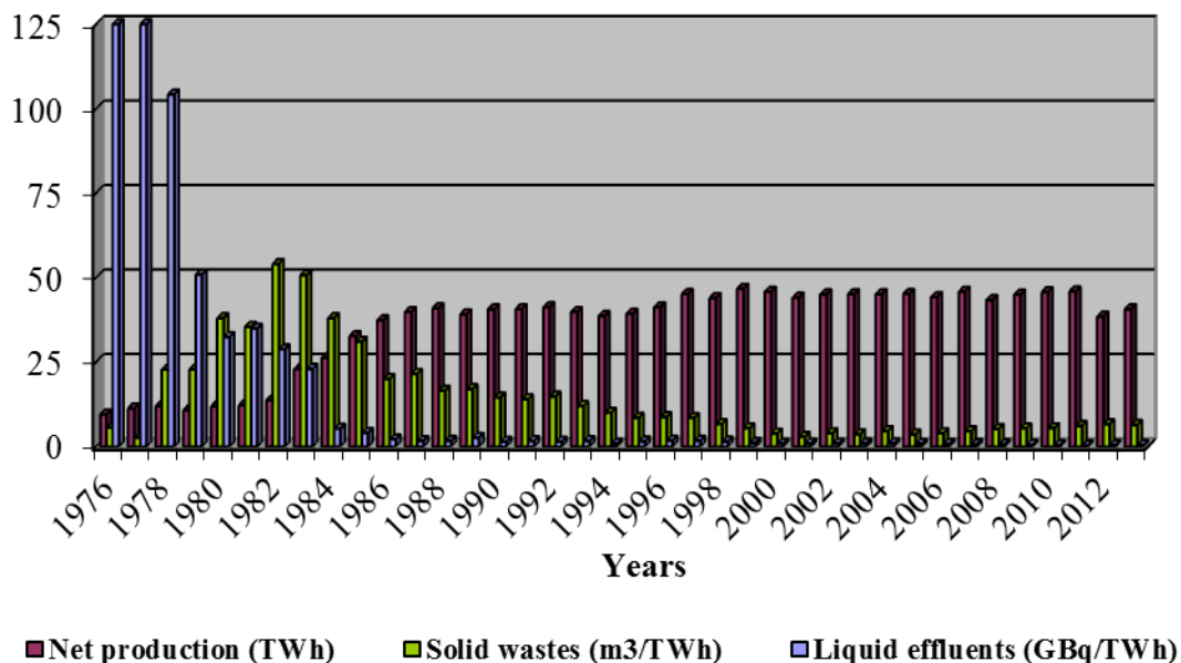
Production of the Belgian nuclear sites (Doel and Tihange NPP)
